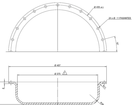
Deep-drawn sheet metal part in 8 mm thickness for industrial valves.
